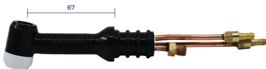
WON 350A 水冷柔性焊枪WT-18F
