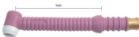
WON350A 风冷柔性加长焊枪WT26FLL 6-83
