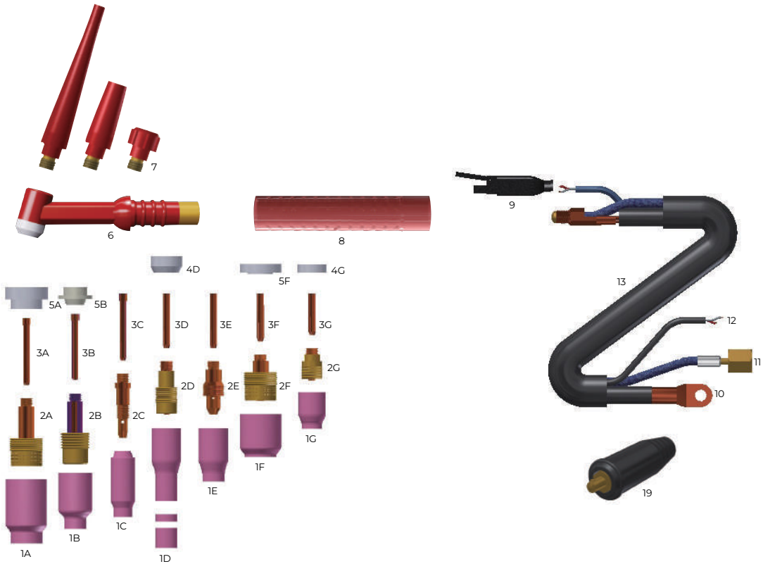
WT26&200A 风冷两件式零件/
