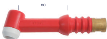
WON350A Air-cooled Flexible Torch WT26FL 6-80
