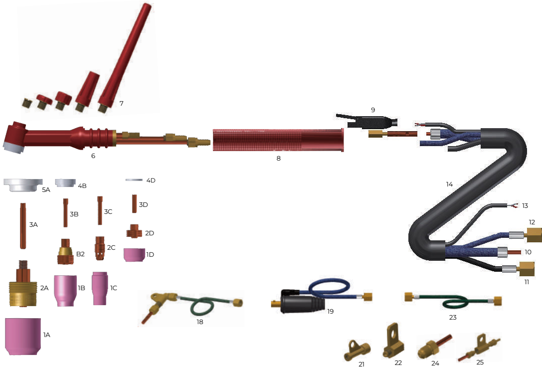
WT20&amp;180A Water-cooled Parts List
