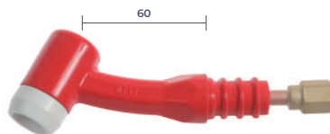
WON170A Air-cooled Flexible Torch WT17F 6-76-1
