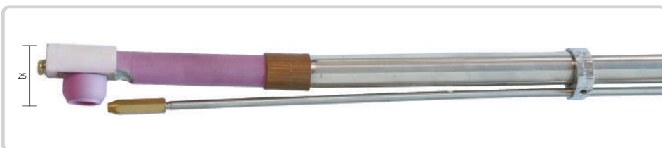
Overlay Welding Torch 32mm in Diameter WT00002 / Overlay Welding Torch 32mm in Diameter WT00002
