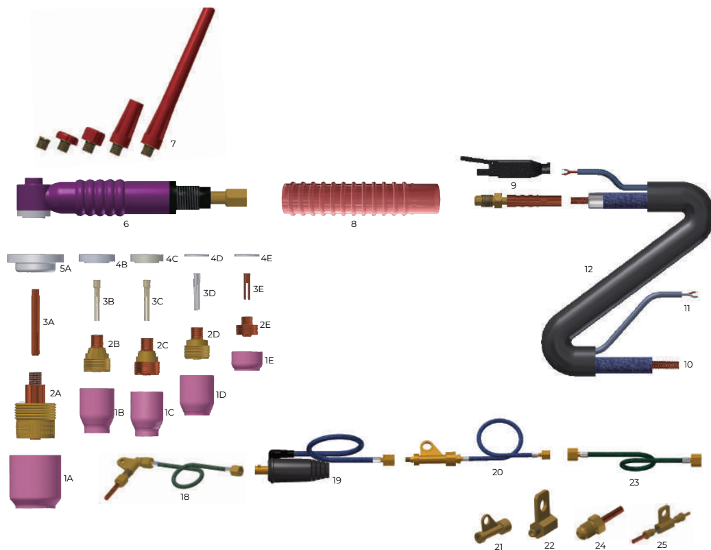
WT80A&125A&150A&170A Air-cooled One-piece Boiler Parts List
