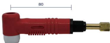
WON 170A Air-cooled Flexible Torch WT-170F
