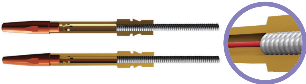
Diffuser for Preventing Solid Wire Short Circuits
