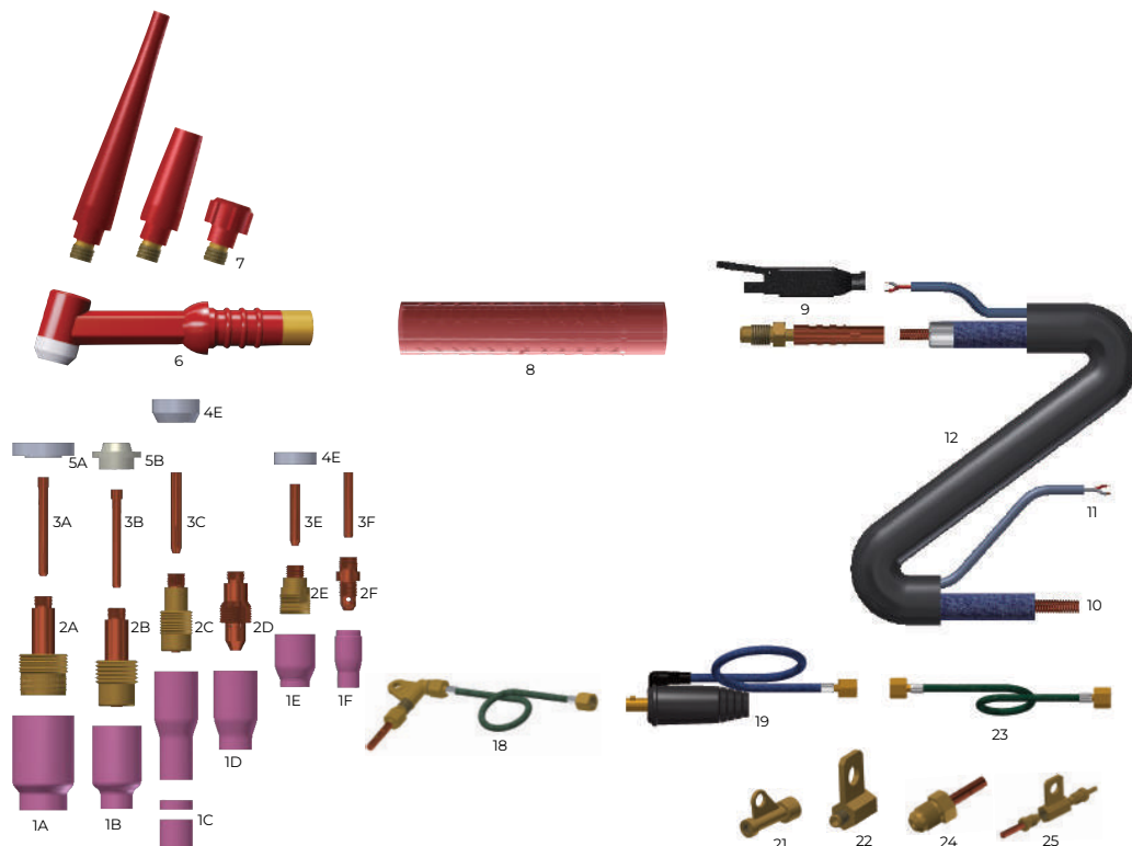
WT26&200A Air-cooled One-piece Parts List
