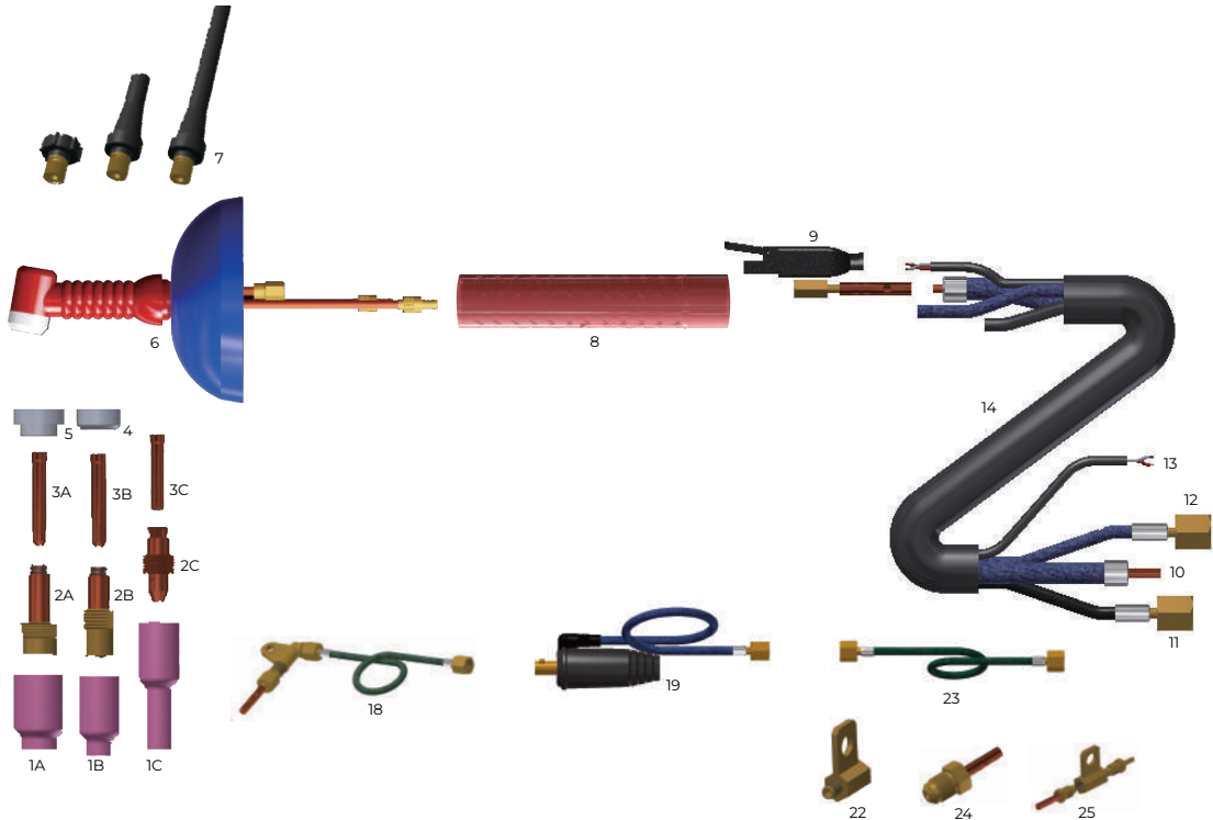
WT40&amp;400A High-capacity Water-cooled Parts List
