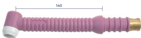
WON350A Air-cooled Flexible Long Torch WT26FLL 6-83
