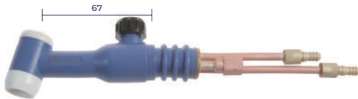
WON350A Water-cooled Valve Torch WT18VW 6-78-1 WON350A 수냉 밸브 토치 WT18VW 6-78-1
