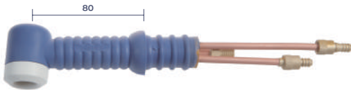
WON400A Water-cooled Flexible Torch WT400FW 40-104-2 WON400A 수냉 후렉시블 토치 WT400FW 40-104-2
