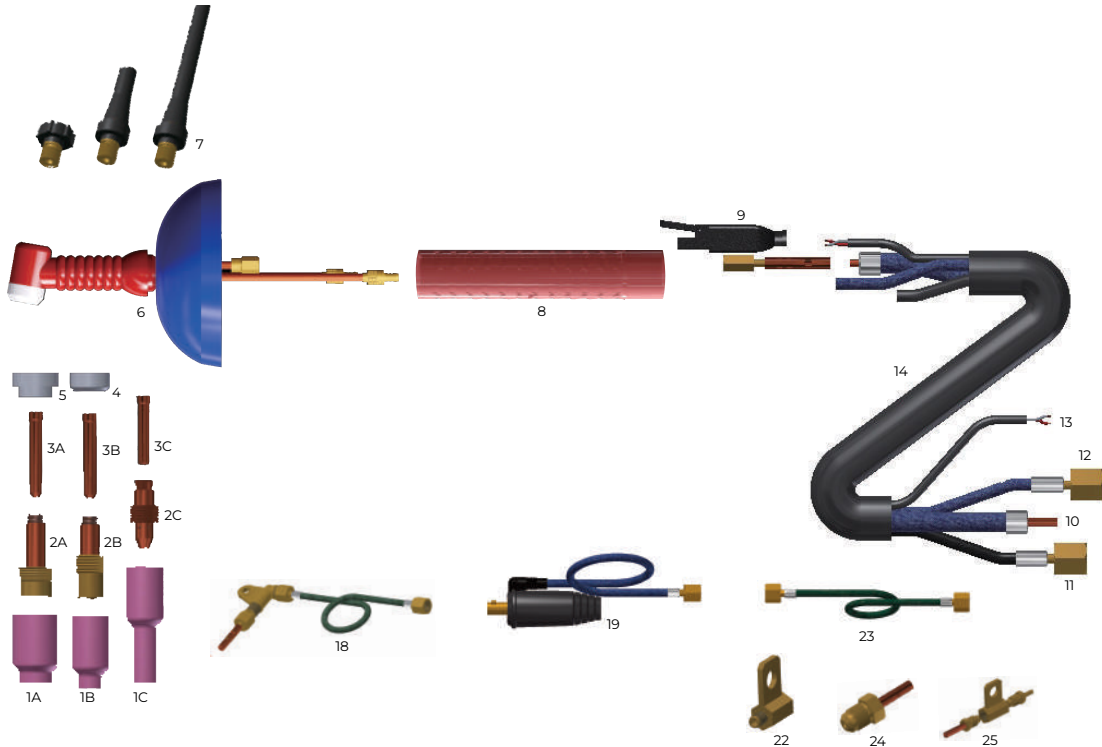
WT40&amp;400A High-capacity Water-cooled Parts / WT40&amp;400A 고용량 수냉 부품 명칭
