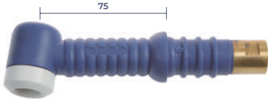
WON400A Air-cooled Flexible Torch WT400F 40-104 WON400A 공냉 후렉시블 토치 WT400F 40-104
