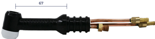
WON 350A Water-cooled Flexible Torch WT-18F WON 350A 수냉 후렉시블 토치 WT-18F
